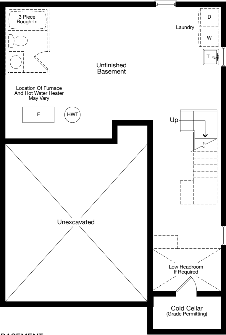
BASEMENT ELEVATION A & B
